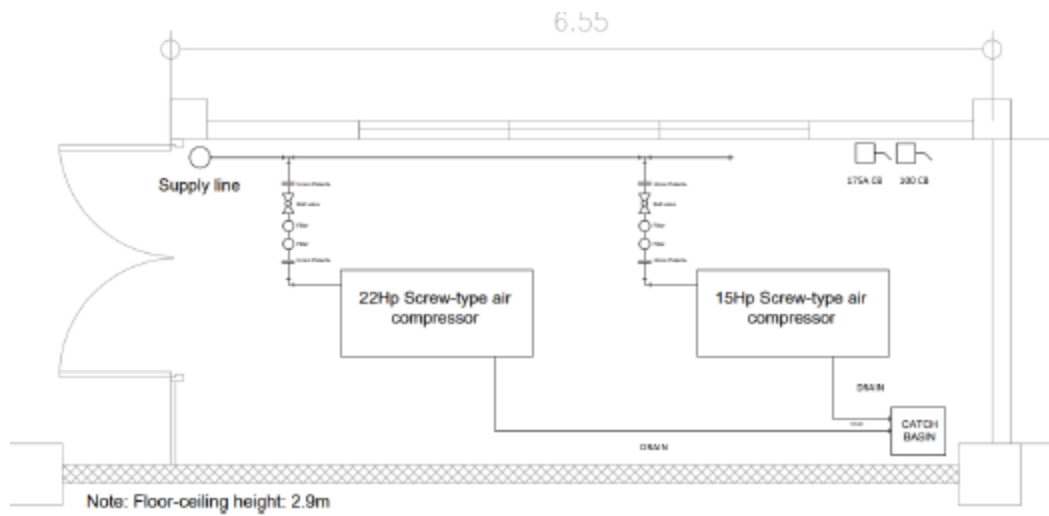
Layout of existing compressor room
