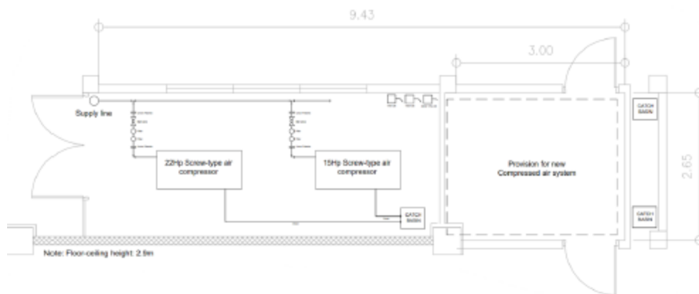
Layout of the new compressor room
